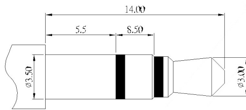
Ø3.50mm 3 POLE PLUG
