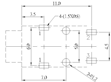
P.C.B LAYOUT MOUNTING PATTERN (TOP VIEW)
