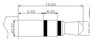
3.5mm 3 POLE PLUG
