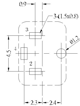
P.C.B LAYOUT MOUNTING PATTERN (TOP VIEW)
