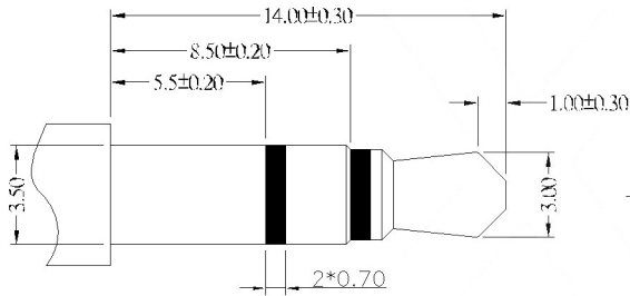
Ø3.50mm 3 POLE PLUG
