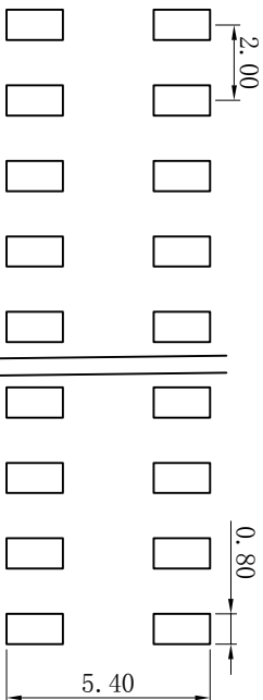
PCB LAYOUT
