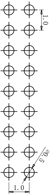
PCB LAYOUT
