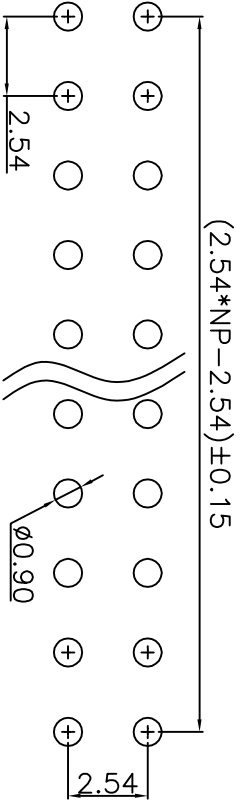
PCB LAYOUT
