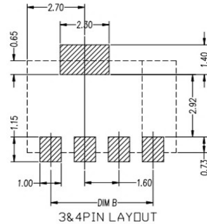
3&4PIN LAYOUT RECOMMENDED PCB LAYOUT TOL:( \pm 0.05 )
