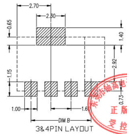
RECOMMENDED PCB LAYOUT TOL:(±0.05)
