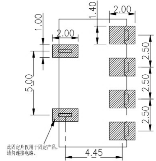
RECOMMENDED PCB LAYOUT TOP VIEW (.XX±0.05)
