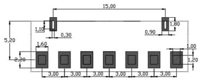
RECOMMENDED PCB LAYOUT TOP VIEW (XX±0.05)
