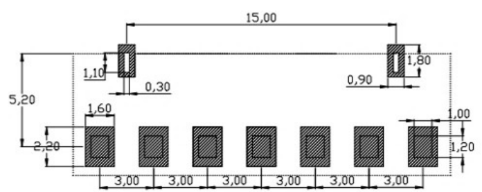
RECOMMENDED PCB LAYOUT TOP VIEW (.XX±0.05)
