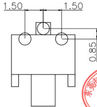
PCB Layout
