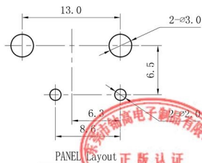
PANEL Layout
