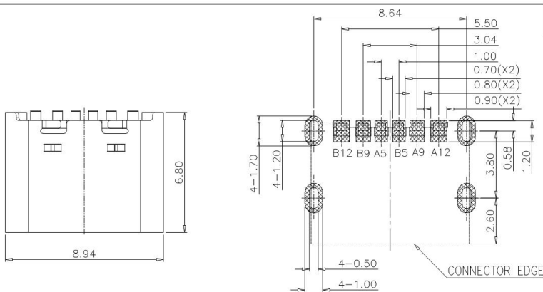
RECOMMENDED PCB LAYOUT(TOP VIEW) THICKNESS 1.6±0.10MM;DEFAULT TOLERANCE:±0.05
